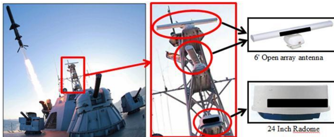
Figure 24 Commercial radar antennas adapted for naval vessel
