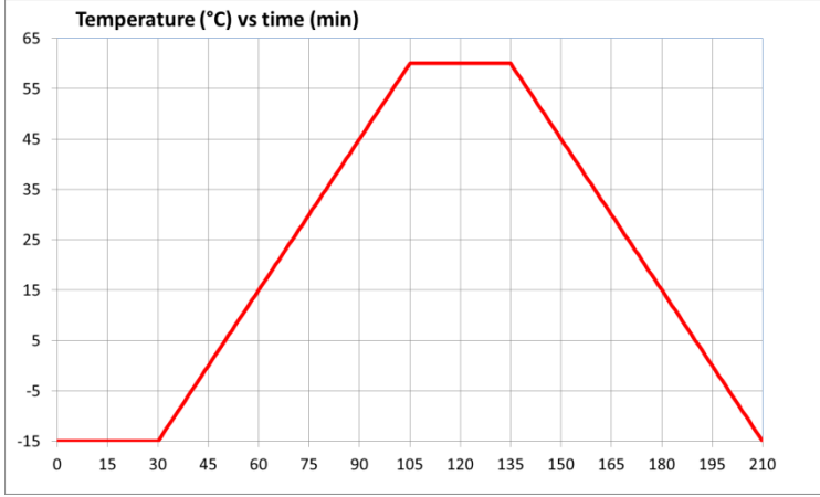
Figure C3/2 Temperature conditioning cycle
