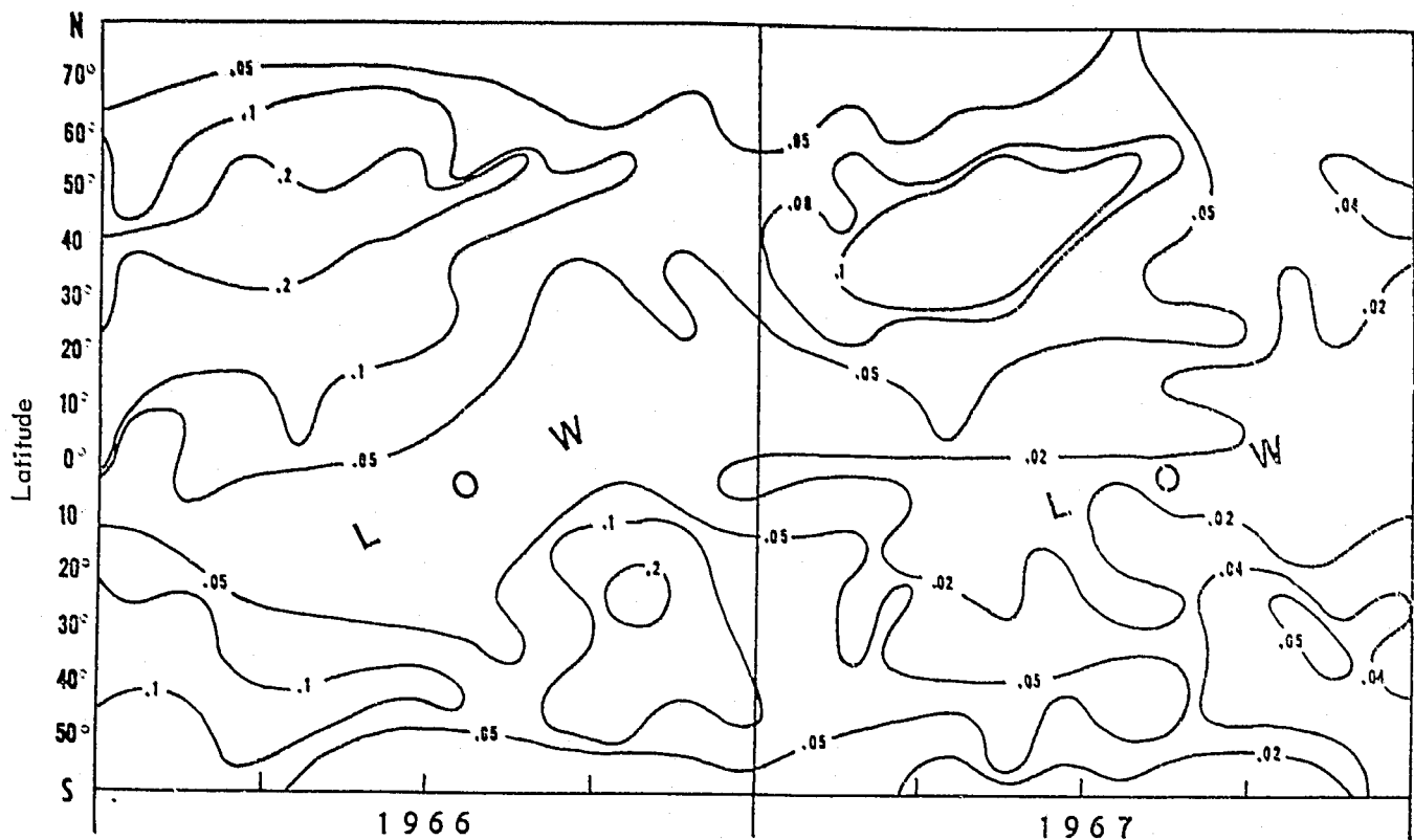
Figure 2. Monthly zonal average deposition of ^{90}\text{Sr} by latitude and time, 1966-1967 44 (mCi km -2 per month)
