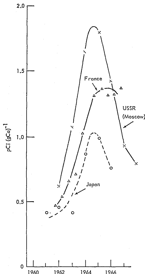
Figure 19. ^{90}\text{Sr}/\text{Ca} ratios in adult ribs
