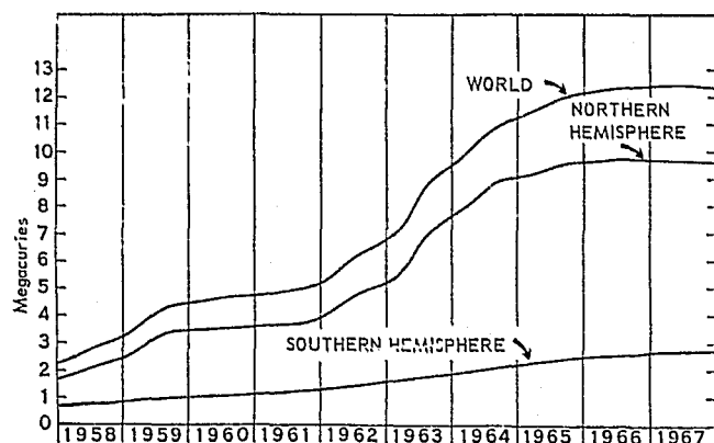
Figure 5. Cumulative ^{90}\text{Sr} deposits 144
