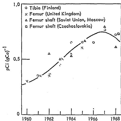
Figure 18. ^{90}\text{Sr}/\text{Ca} ratios in long bones
