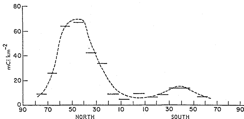
Figure 13. Average latitudinal distribution of deposited ^{90}\text{Sr} from analyses of soils collected 1965-1967 90
