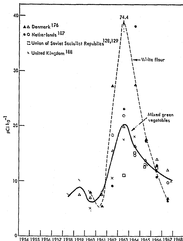
Figure 15. ^{90}\text{Sr} content of green vegetables and white flour in the north temperate zone
