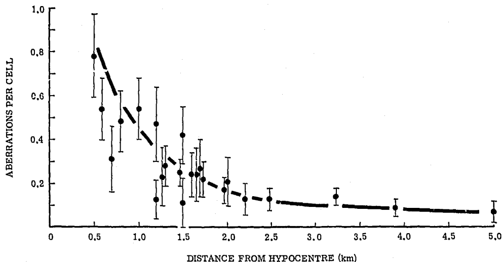
Figure 15. Number of dicentrics plus rings per X_1Cu cell versus distance from hypocentre 221
