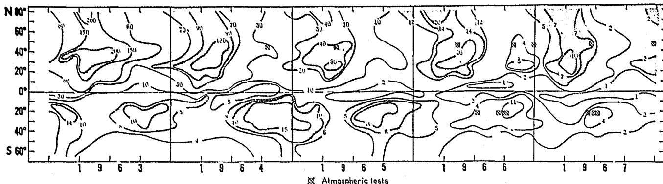
Figure 4. ^{90}\text{Sr} concentrations in surface air based on observations made between 35^\circ\text{W} and 155^\circ\text{W} 175 (dpm per 1,000 scm, where 1 scm = 1.226 kg air)
